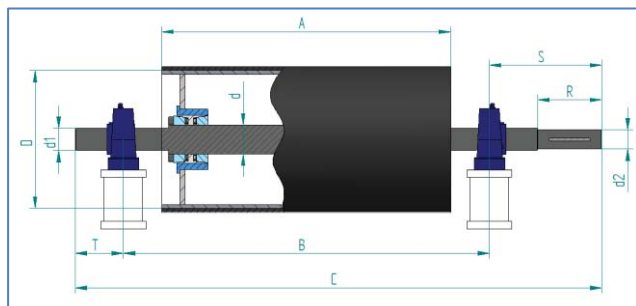
Shaft with clamping units
